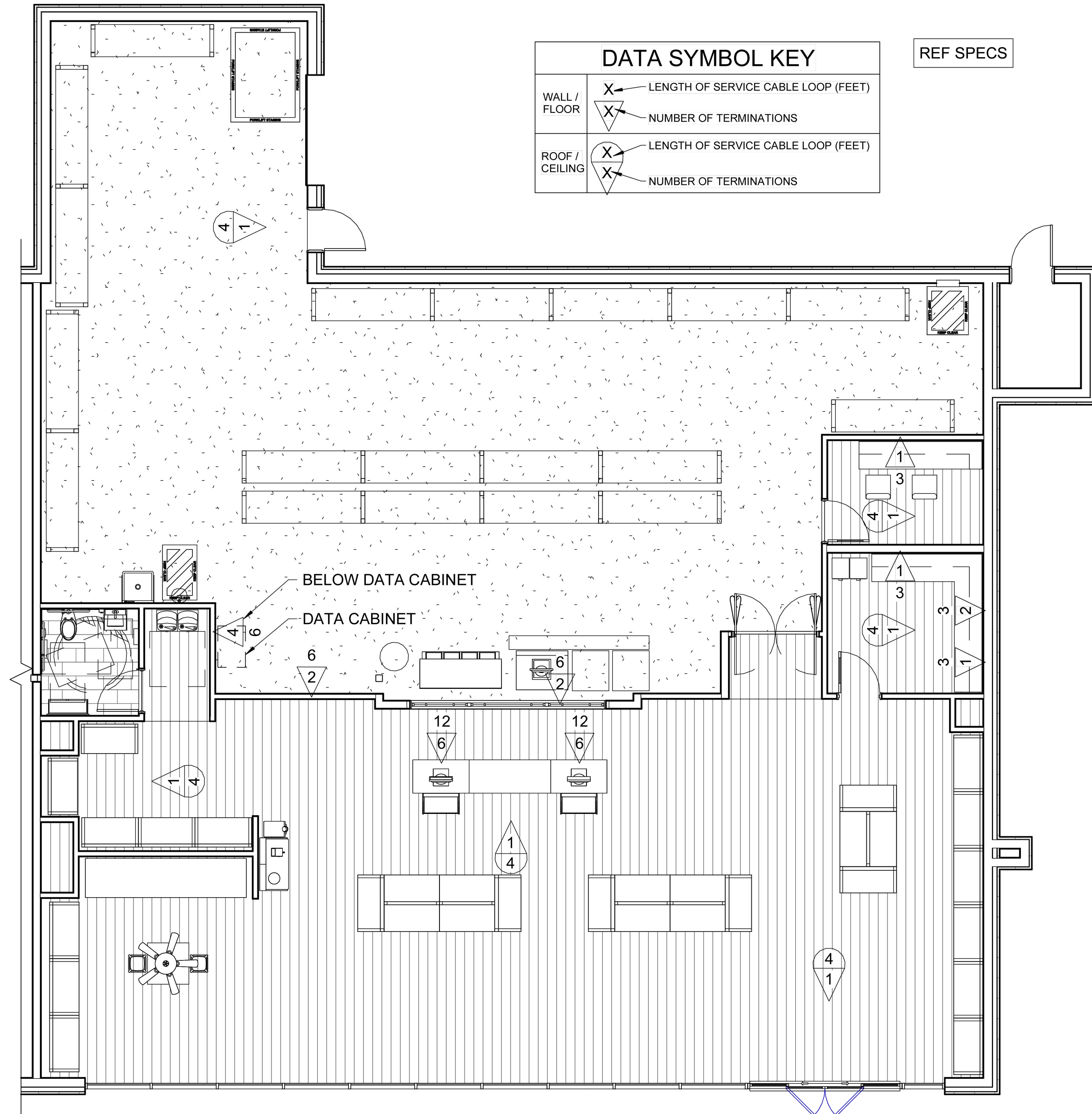
1 STRUCTURED CABLING LOCATION SCALE: N.T.S.
