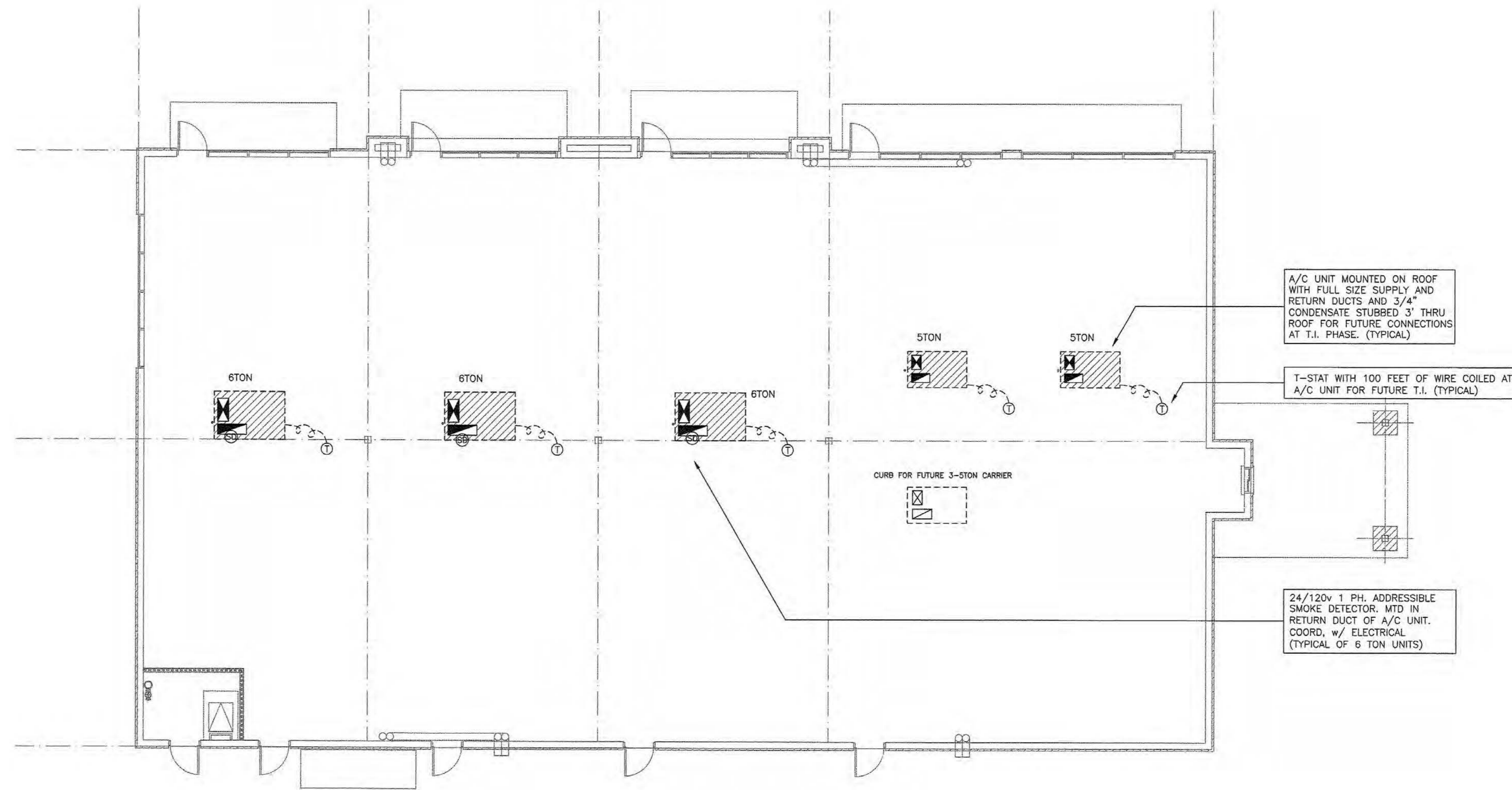
MECHANICAL FLOOR PLAN 1/8"=1'-0" NORTH
